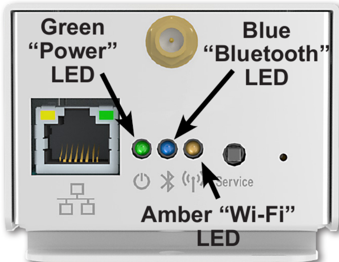
Fig. 11: Gateway LEDs
