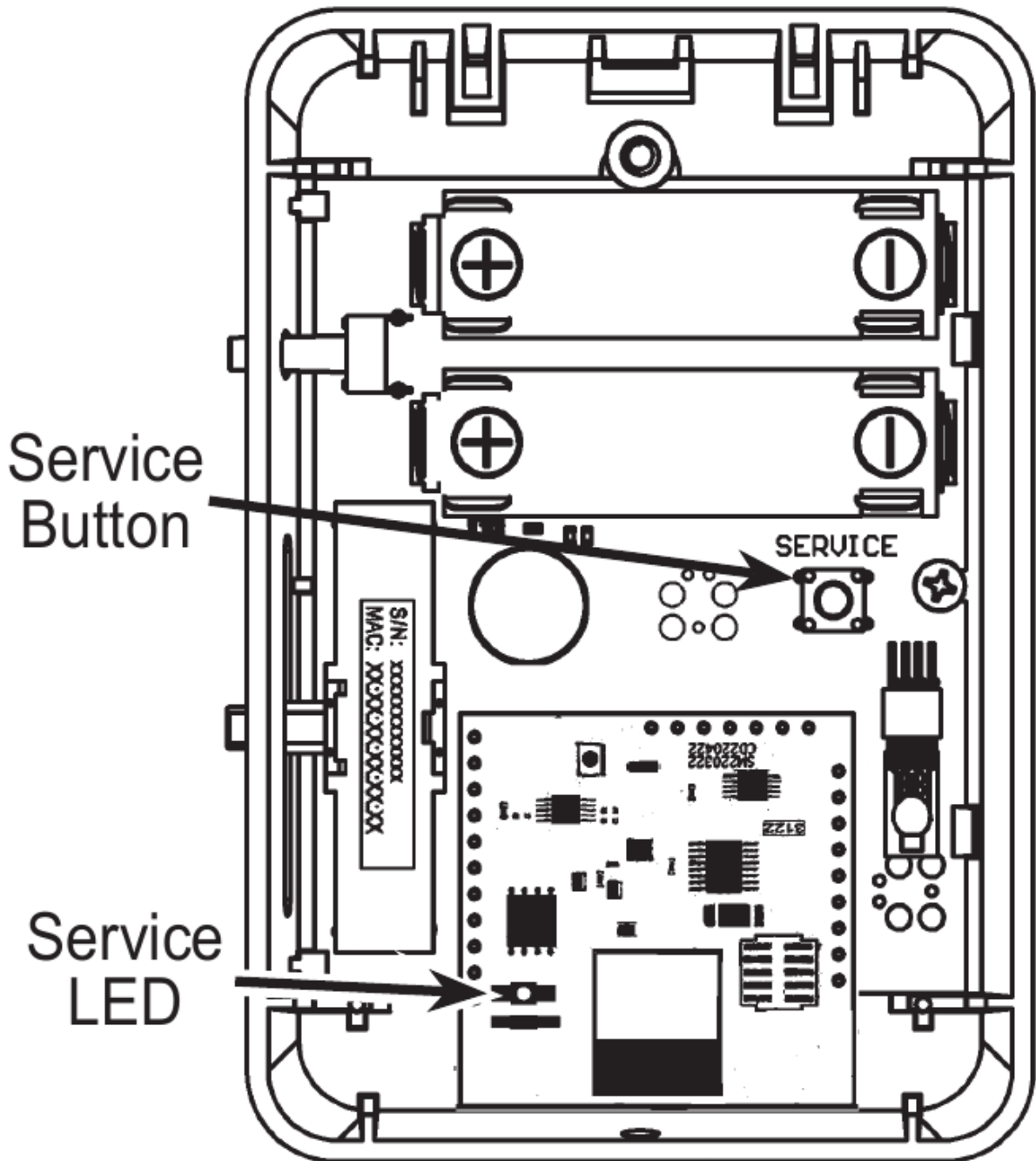
Fig. 9: BAPI-Stat "Quantum" Sensor Service Button and LED
