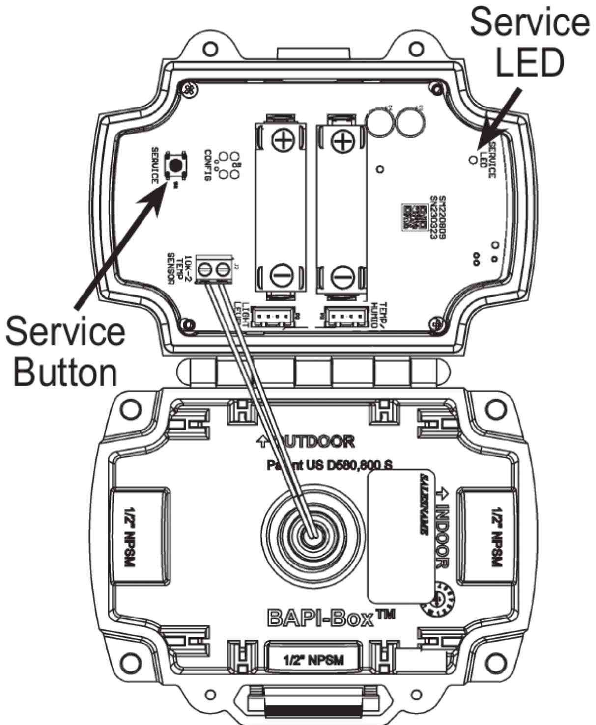
Fig. 8: BAPI-Box Sensor Service Button and LED
