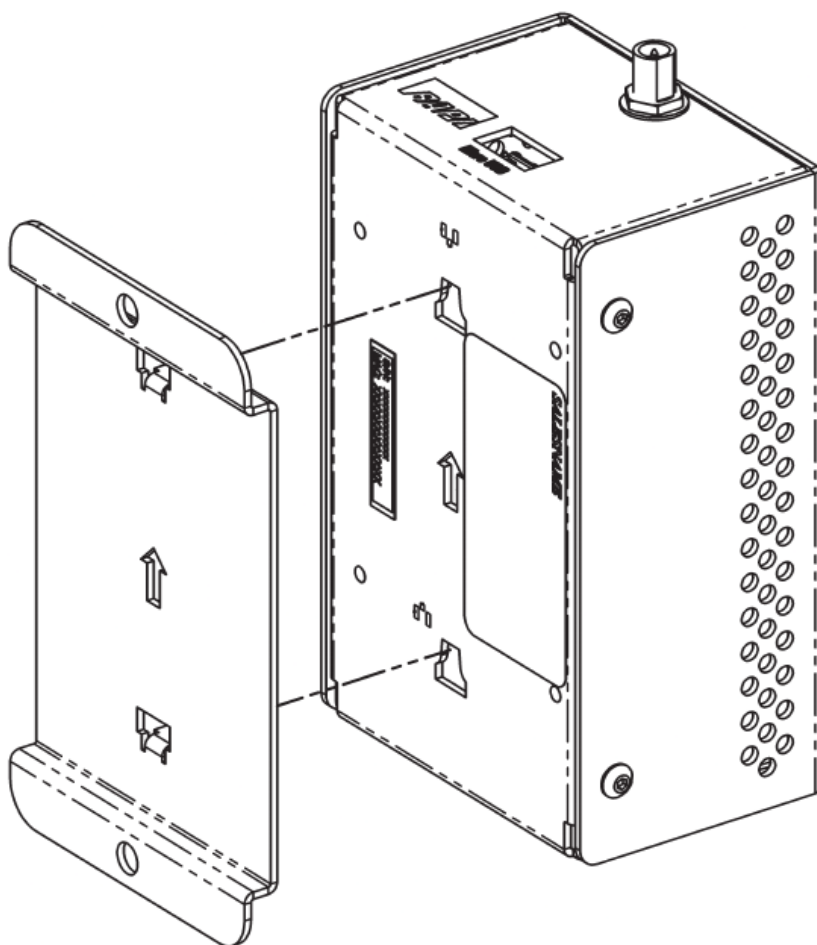
Fig. 10: Gateway mounting
