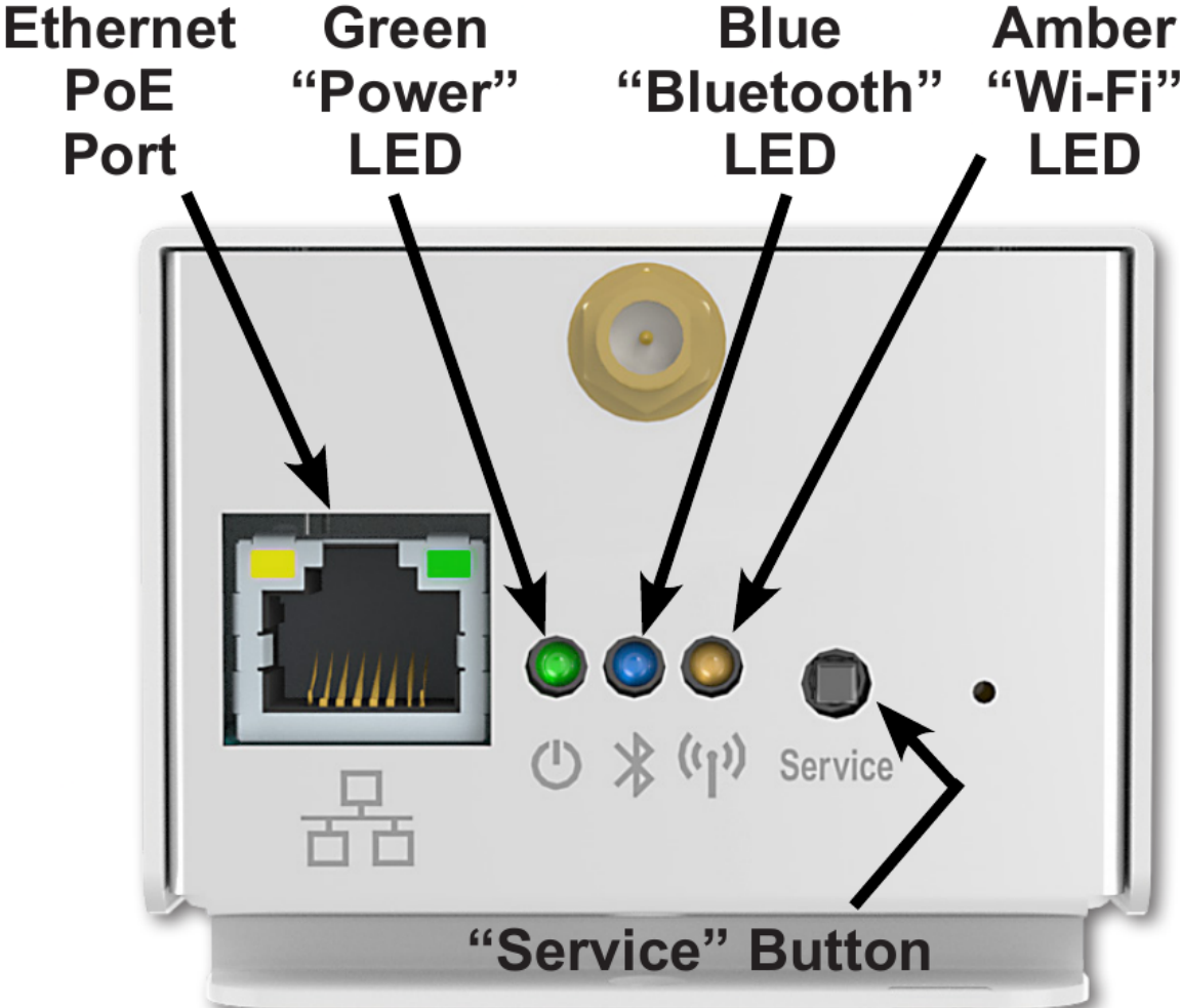
Fig. 1: Gateway PoE Port and LEDs
