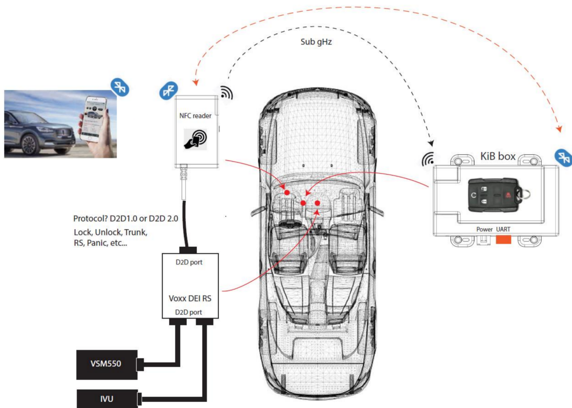
Figure 1 EKey System Diagram
